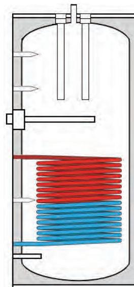
SINGLE COIL SOLAR TANK WITH ELECTRICAL BACK UP HEATING
