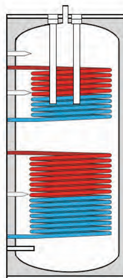
DUAL COIL SOLAR TANK FOR BOILER BACK UP HEATING
